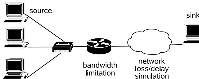
Figure 4.4: Network topology
